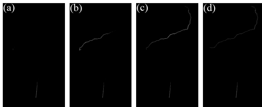
Fig. 1 The distributions of simulated total charge density in different time: (a) 20th minute, (b) 30th minute, (c) 60th minute, (d) 90th minute. The contour lines are isotherms (unit: ^{\circ}\text{C} ).
