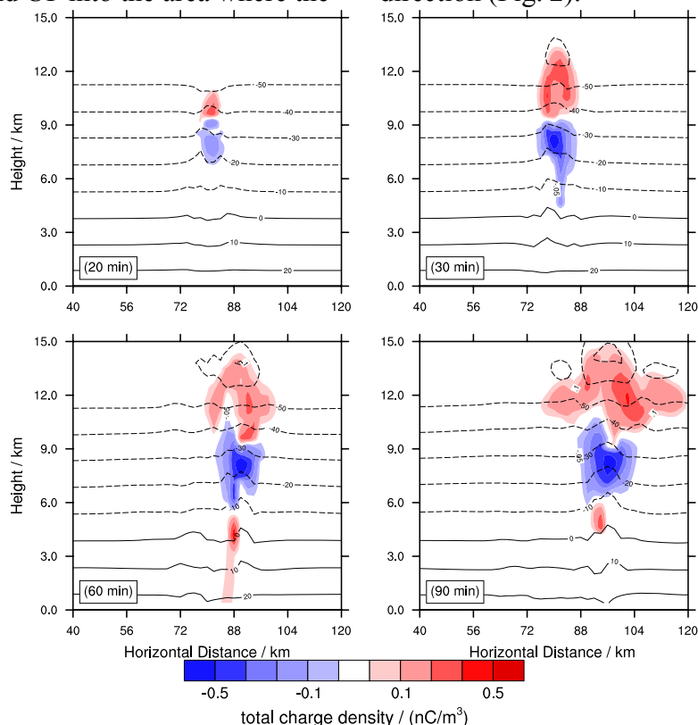
Fig. 1 The distributions of simulated total charge density in different time: (a) 20th minute, (b) 30th minute, (c) 60th minute, (d) 90th minute. The contour lines are isotherms (unit: ^{\circ}\text{C} ).
