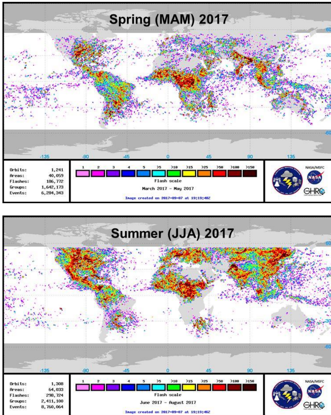
Figure Caption: These figures show the seasonal global lightning detections from LIS on ISS during its first 6 months on orbit. These preliminary results are in good agreement with similar results from OTD and TRMM LIS as a similar point in their mission.
